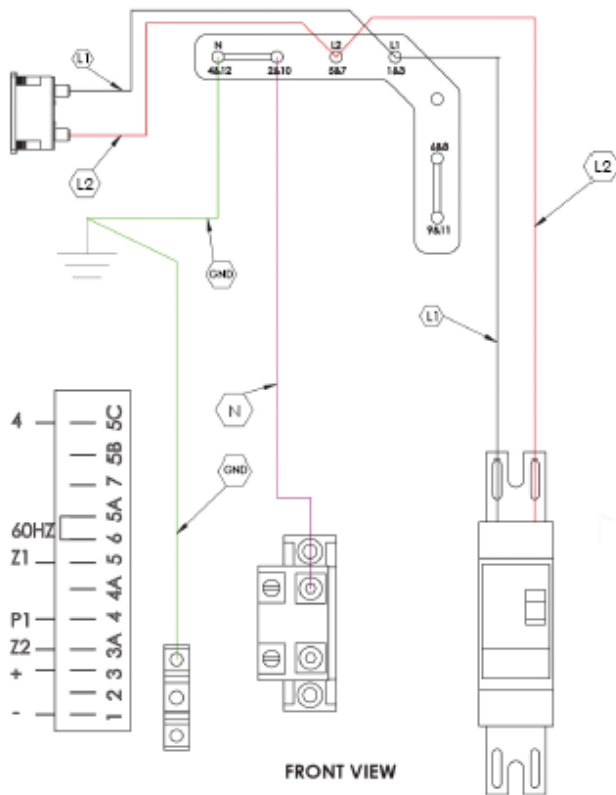
120/240 SINGLE PHASE
