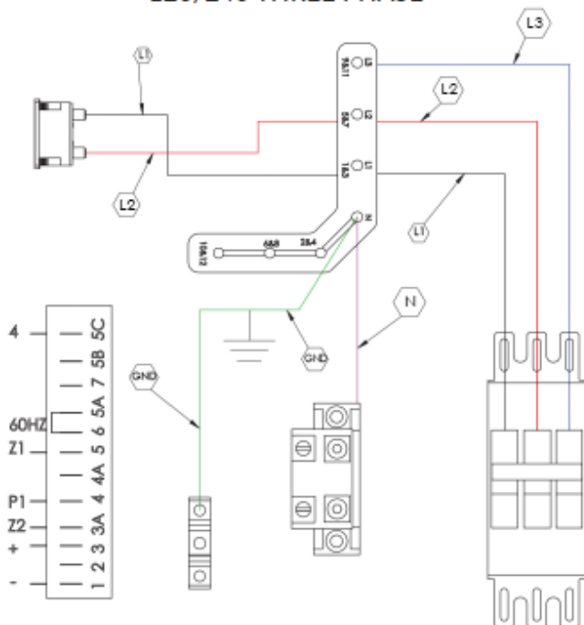
120/240 THREE PHASE
