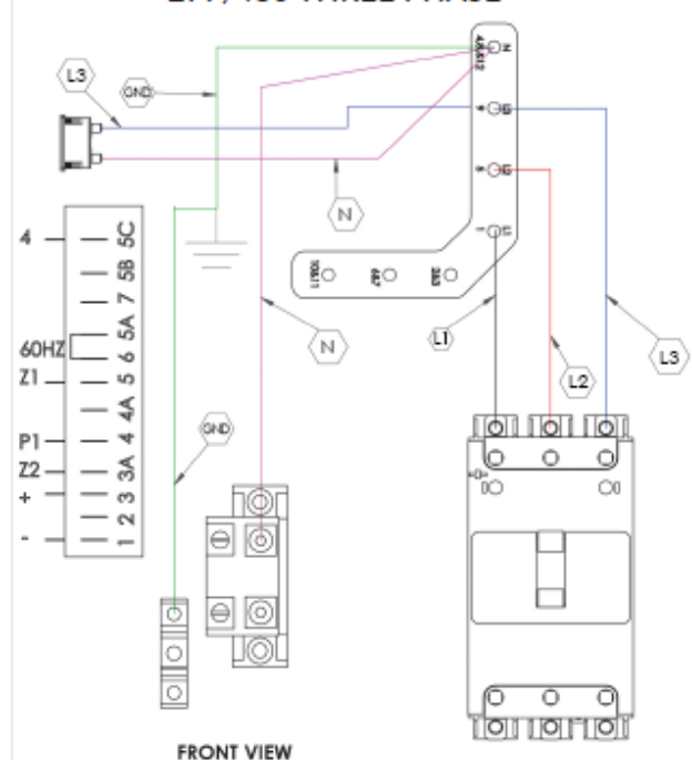
277/480 THREE PHASE
