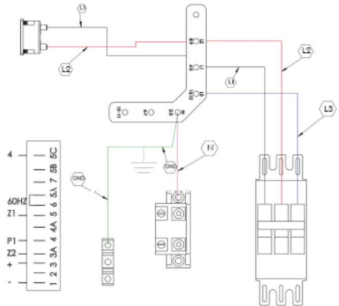
120/208 THREE PHASE
